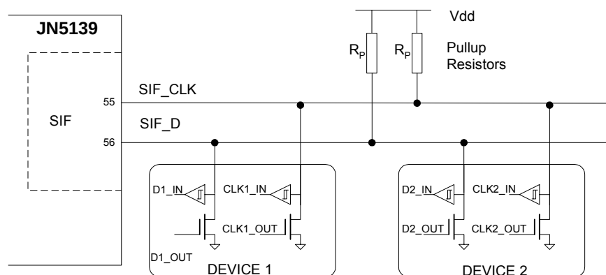
Figure 36 Connection Details
