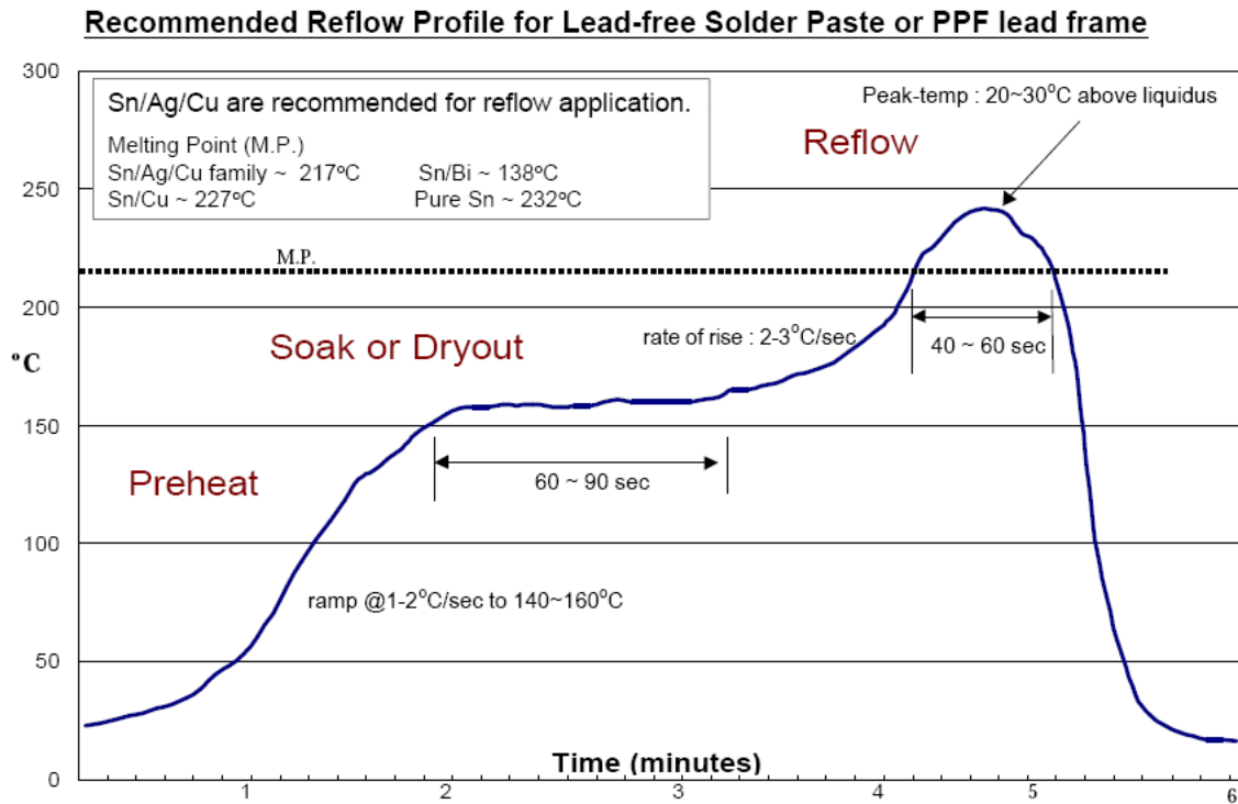
Figure 48: Reflow Profile
