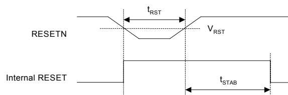
Figure 41: External Reset
